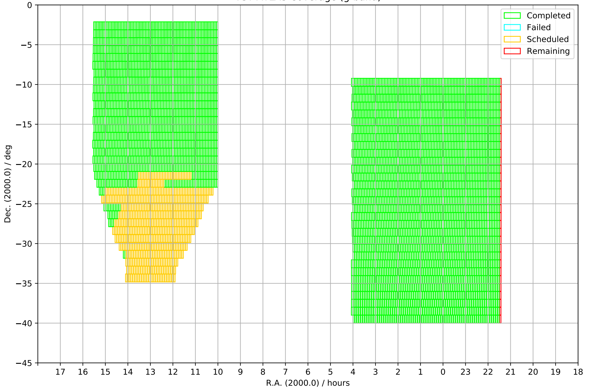
VST ATLAS Coverage (g-band)
