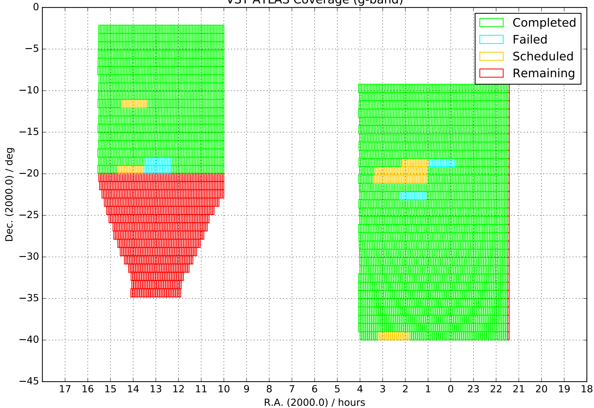
VST ATLAS Coverage (g-band)
