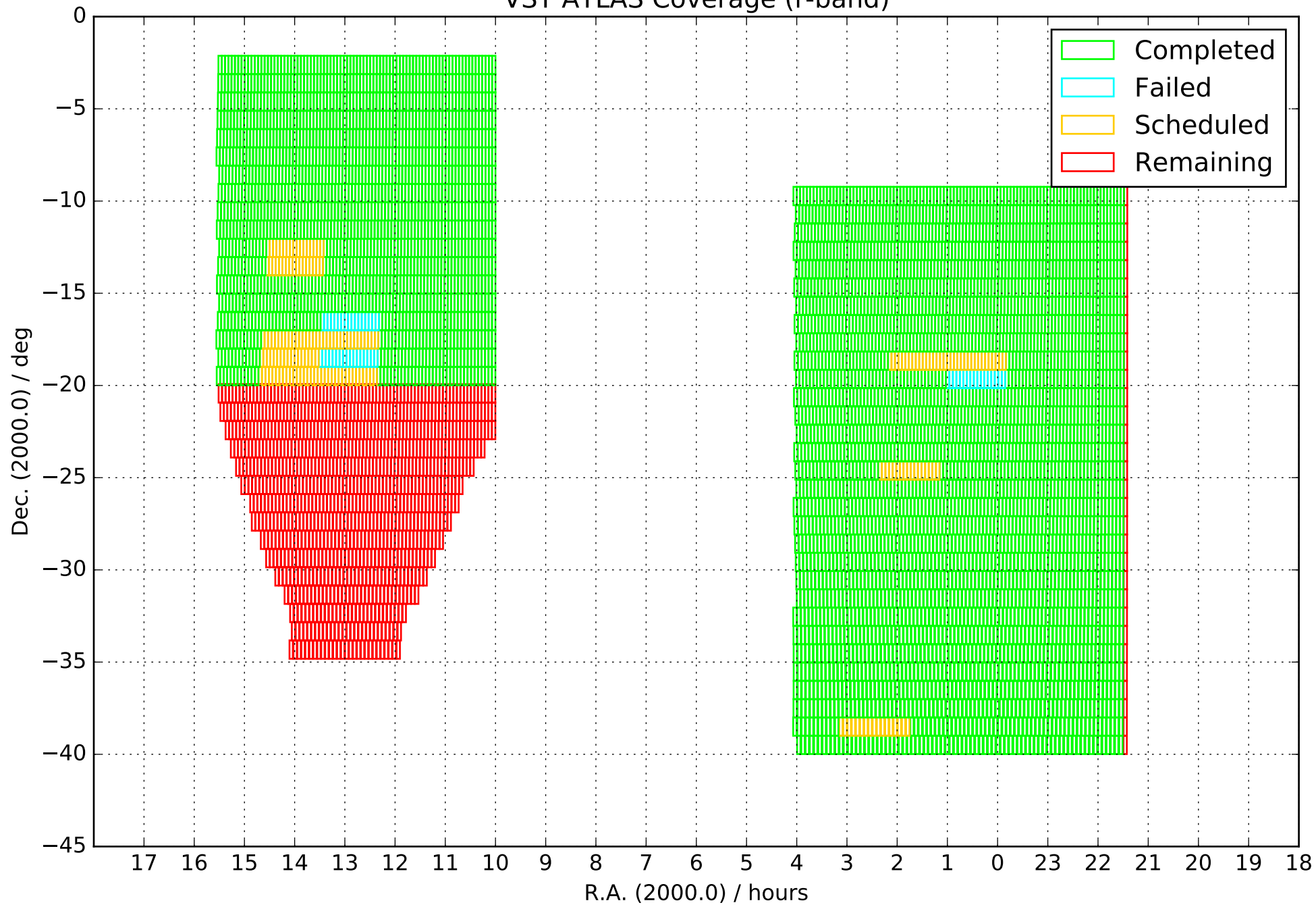
VST ATLAS Coverage (r-band)
