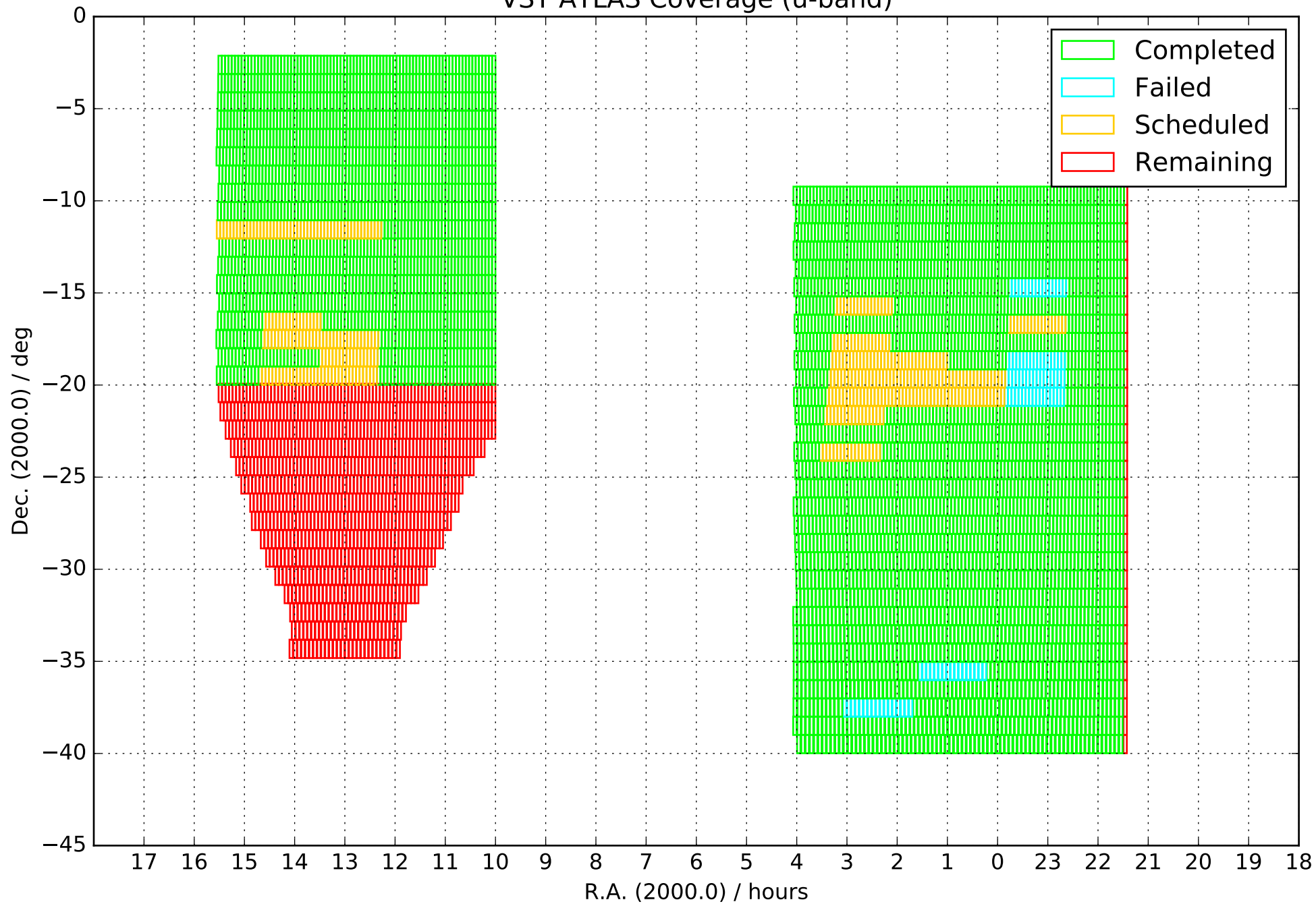
VST ATLAS Coverage (u-band)
