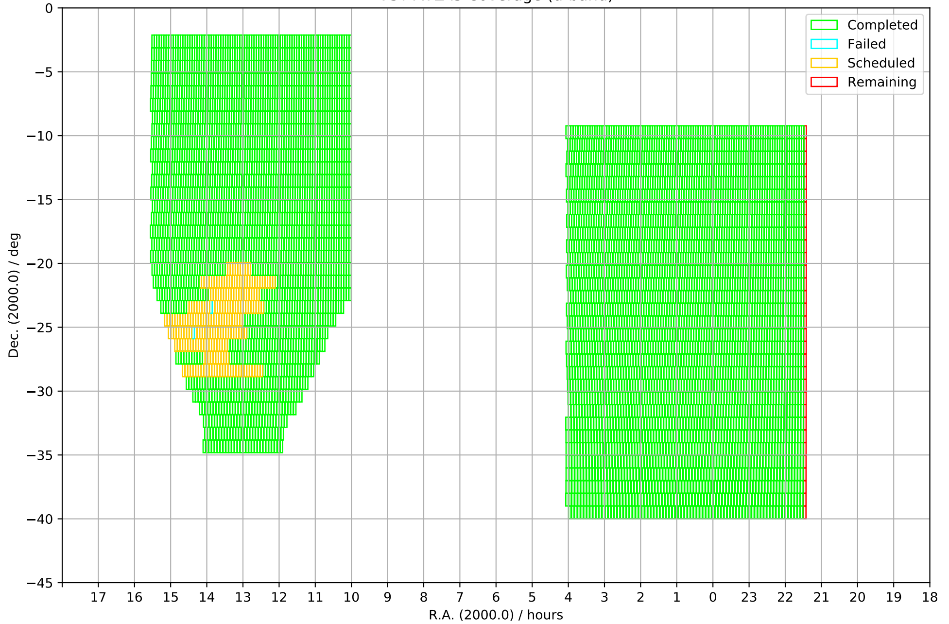
VST ATLAS Coverage (u-band)
