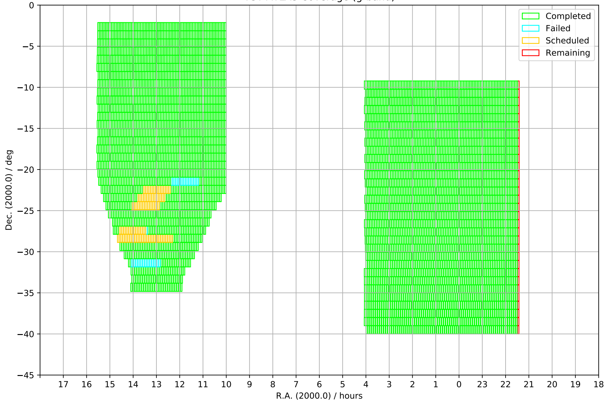
VST ATLAS Coverage (g-band)
