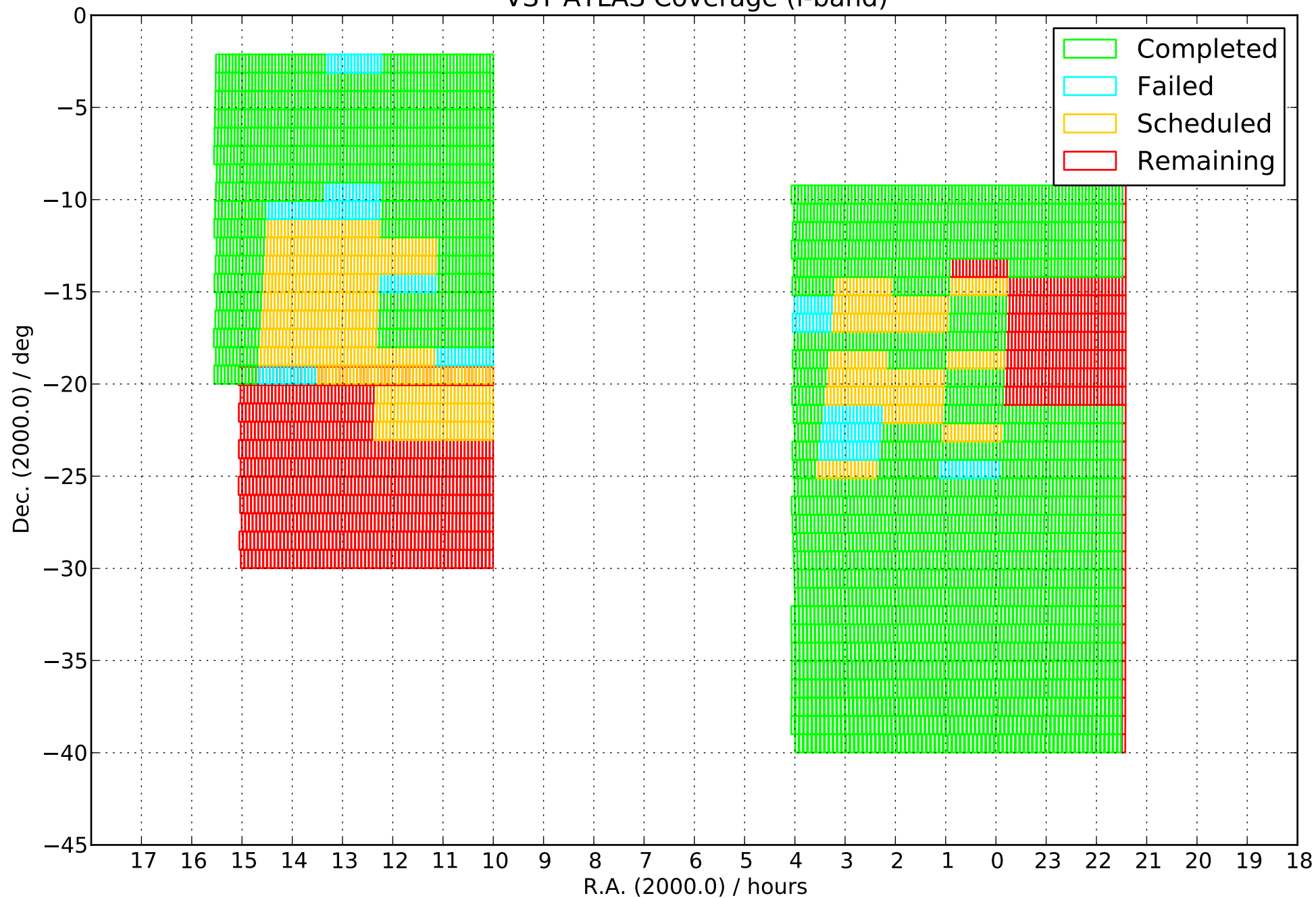
VST ATLAS Coverage (i-band)
