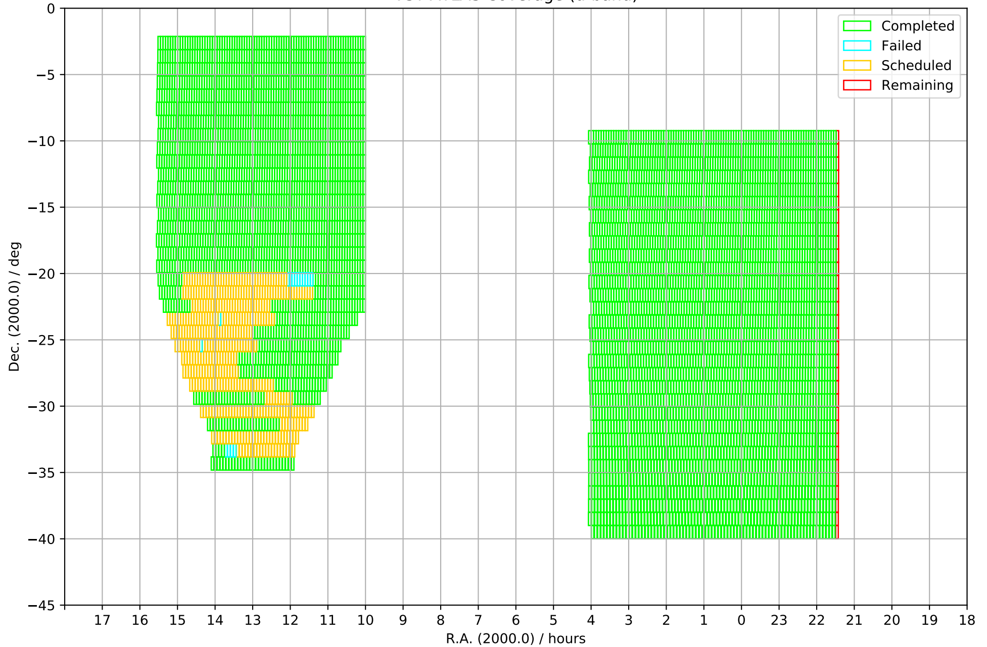
VST ATLAS Coverage (u-band)
