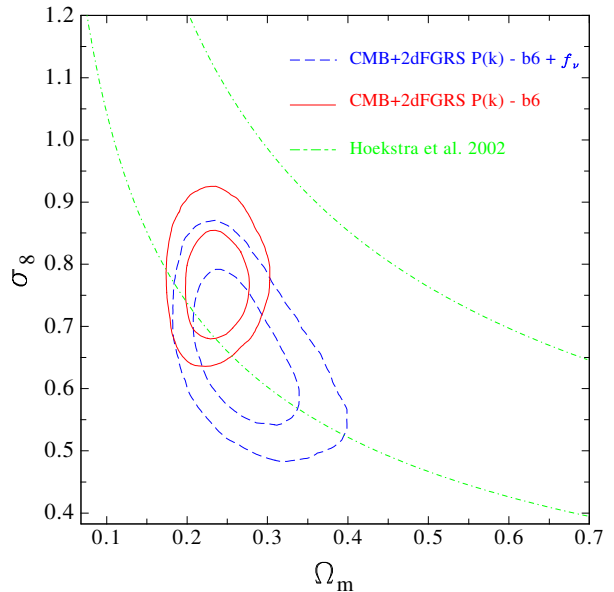
Figure 12. The marginalized posterior likelihood in the \Omega_m - \sigma_8 plane obtained using CMB plus 2dFGRS information for different parameter sets. The solid lines correspond to the 68% and 95% contours obtained for the basic-six parameter set. The dashed lines correspond to the results obtained when the neutrino fraction f_\nu is also allowed to vary. The dot-dashed lines show constraints from weak lensing measurements from Hoekstra et al. (2002).
