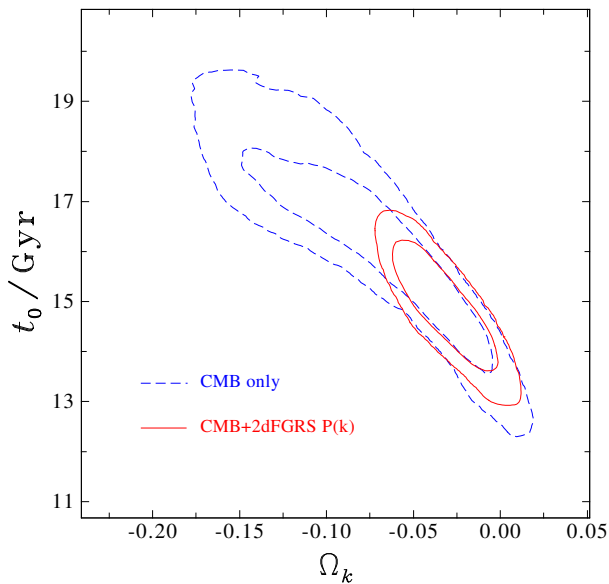
Figure 14. The marginalized posterior likelihood in the \Omega_k - t_0 plane for the basic-six plus \Omega_k parameter set. The dashed lines show the 68% and 95% contours obtained in the CMB only case. The solid contours correspond to the constraints obtained in the CMB plus 2dFGRS case.
