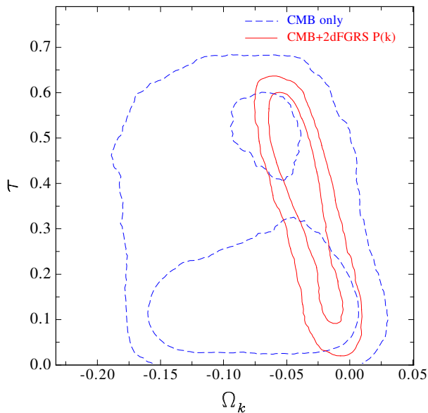
Figure 6. The marginalized posterior likelihood in the \Omega_k - \tau plane for the basic-six plus \Omega_k parameter set. The dashed lines show the 68% and 95% contours obtained in the CMB only case. The solid contours correspond to the constraints obtained in the CMB plus 2dFGRS P(k) case.
