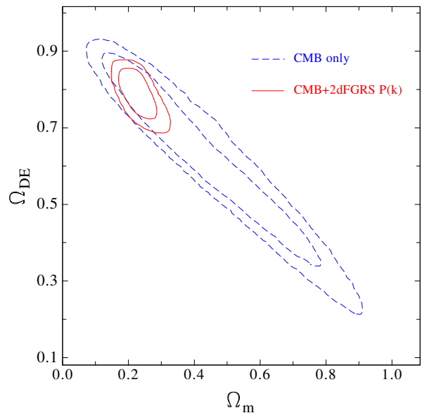
Figure 7. The marginalized posterior likelihood in the \Omega_m - \Omega_{DE} plane for the basic-six plus \Omega_k parameter set. The dashed lines show the 68% and 95% contours obtained in the CMB only case. The solid contours correspond to constraints in the CMB plus 2dFGRS P(k) case.
