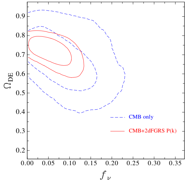
Figure 4. The marginalized posterior likelihood in the f_\nu - \Omega_{\text{DE}} plane for the basic-six+ f_\nu parameter set. The dashed lines show the 68% and 95% contours obtained in the CMB only case. The solid contours show the parameter constraints obtained for combined CMB and 2dFGRS P(k) datasets.
