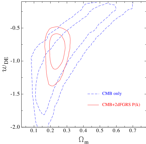
Figure 8. The marginalized posterior likelihood in the \Omega_m - w_{\text{DE}} plane for the basic six plus w_{\text{DE}} parameter set. The dashed lines show the 68% and 95% contours obtained in the CMB only case. The solid contours show the corresponding constraints obtained in the CMB+2dFGRS P(k) case.
