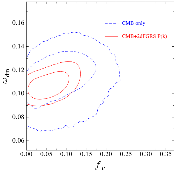
Figure 3. The marginalized posterior likelihood in the f_\nu - \omega_{\text{dm}} plane for the basic-six+ f_\nu parameter set. The dashed lines show the 68% and 95% contours obtained in the CMB only case. The solid contours show the corresponding results obtained in the CMB plus 2dFGRS P(k) case.
