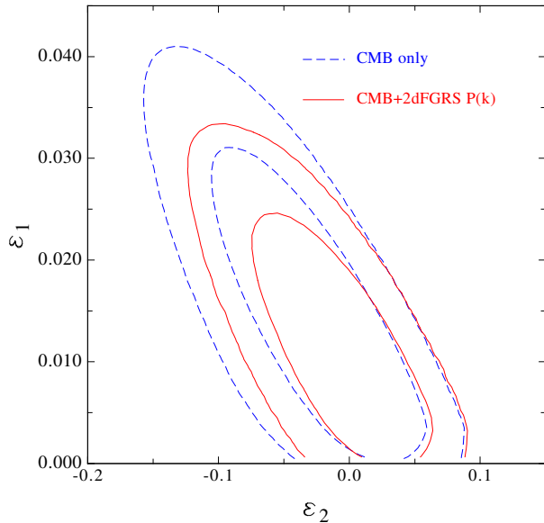
Figure 10. The marginalized posterior likelihood in the \epsilon_1 - \epsilon_2 plane for the basic-six plus r parameter set. The dashed lines show the 68% and 95% contours obtained in the CMB only case. The solid contours correspond to the results obtained in the CMB plus 2dFGRS P(k) case.
