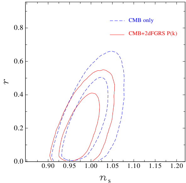
Figure 9. The marginalized posterior likelihood in the n_s - r plane for the basic-six plus r parameter set. The dashed lines show the 68% and 95% contours obtained in the CMB only case. The solid contours show the corresponding results in the CMB plus 2dFGRS P(k) case.
