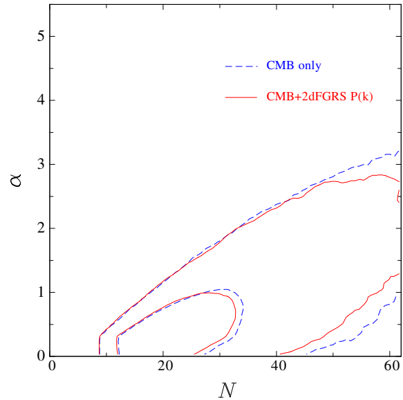
Figure 11. The marginalized posterior likelihood in the \alpha - N plane for the basic-six plus r parameter set. The dashed lines show the 68% and 95% contours obtained in the CMB only case. The solid contours show the results in the CMB plus 2dFGRS P(k) case.
