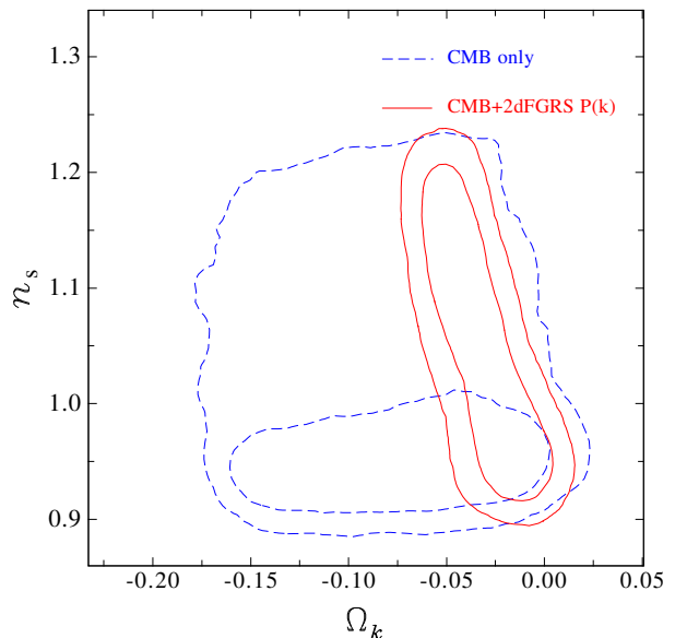
Figure 15. The marginalized posterior likelihood in the \Omega_k - n_s plane for the basic six plus \Omega_k parameter set. The dashed lines show the 68% and 95% contours obtained in the CMB only case. The solid contours correspond to the constraints obtained in the CMB plus 2dFGRS case.
