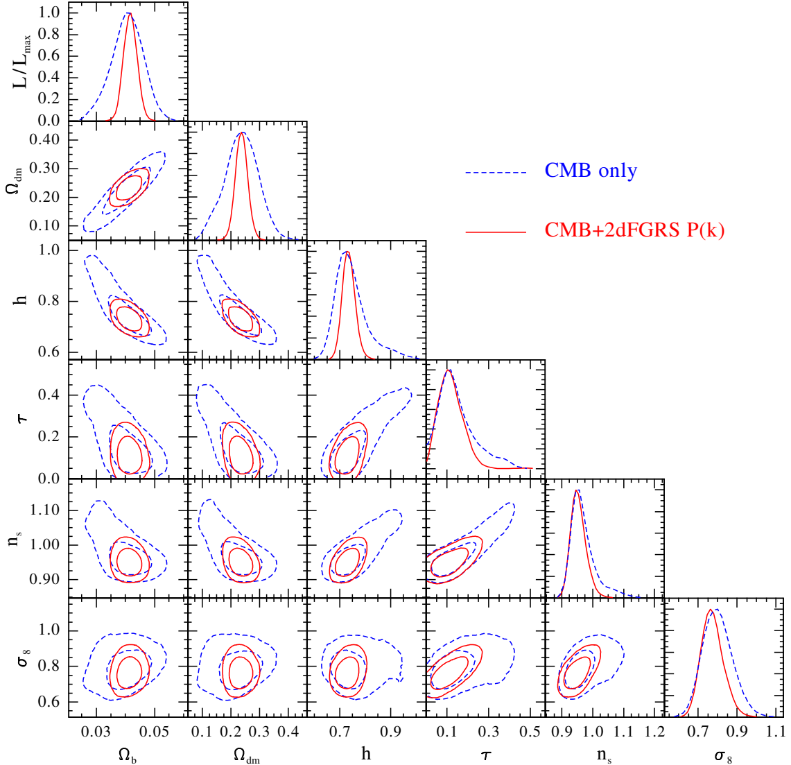
Figure 2. Marginalized posterior likelihoods for the cosmological parameters in the basic-six model determined from CMB information only (dashed lines) and CMB plus 2dFGRS P(k) (solid lines).
