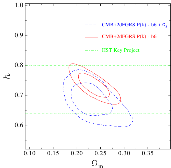
Figure 13. The marginalized posterior likelihood in the \Omega_m - h plane obtained using CMB plus 2dFGRS information for different parameter sets. The solid lines correspond to the 68% and 95% contours obtained for the basic-six parameter set. The dashed lines show the results obtained when non-flat models are considered (basic-six plus \Omega_k ). The dot-dashed lines show the constraint on h from the HST Key Project (Freedman et al. 2001).
