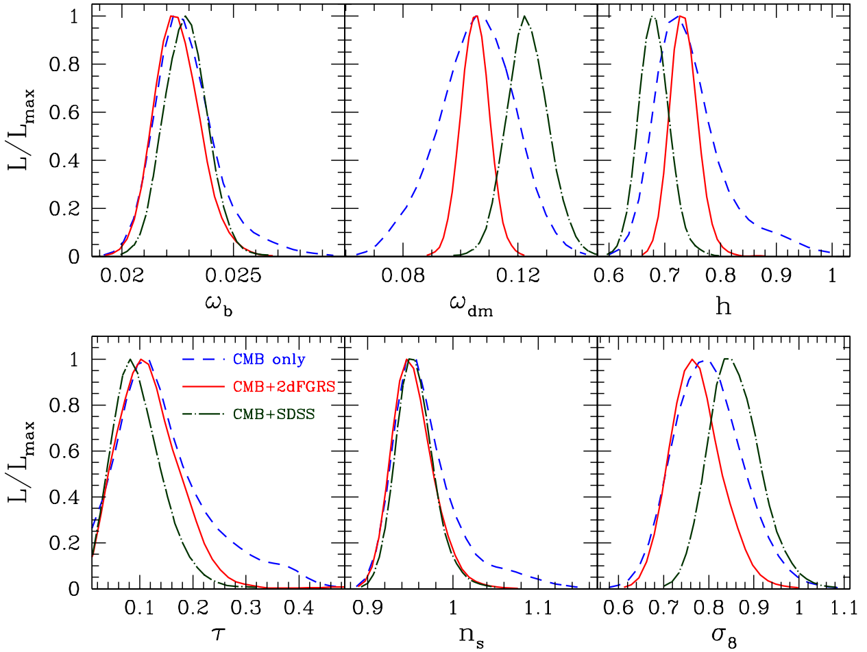
Figure 18. The marginalized one-dimensional posterior likelihood in the basic-six parameter space obtained for CMB information only (dashed lines), CMB plus the 2dFGRS P(k) (solid lines) and CMB plus the SDSS (dot-dashed lines).
