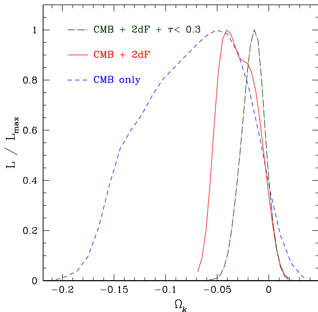
Figure 5. The one dimensional marginalized posterior likelihood for \Omega_k for CMB data only (dashed line), CMB plus 2dFGRS P(k) (solid line), and CMB plus 2dFGRS P(k) , with a prior on the optical depth of \tau < 0.3 (dot-dashed line). Closed models have \Omega_k < 0 .
