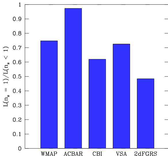
Figure 17. The likelihood ratios of the basic-five model to the basic-six model plotted in Fig.16 for the individual datasets used in our analysis.
